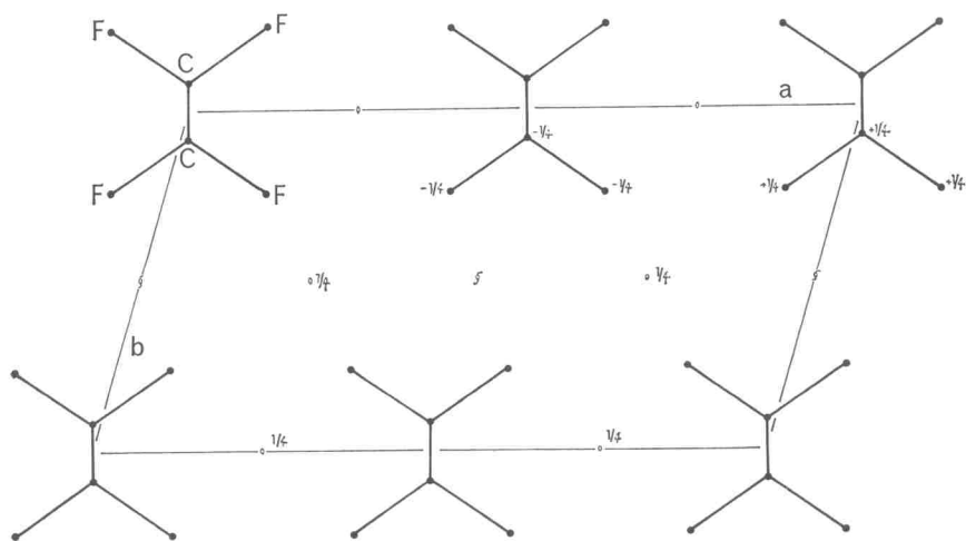
Fig. 7. (001) projection of phase III of PTFE.
